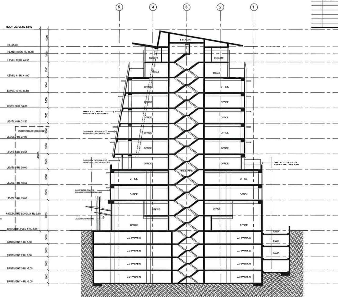
SECTION B - B Scale 1:200 @ A1
