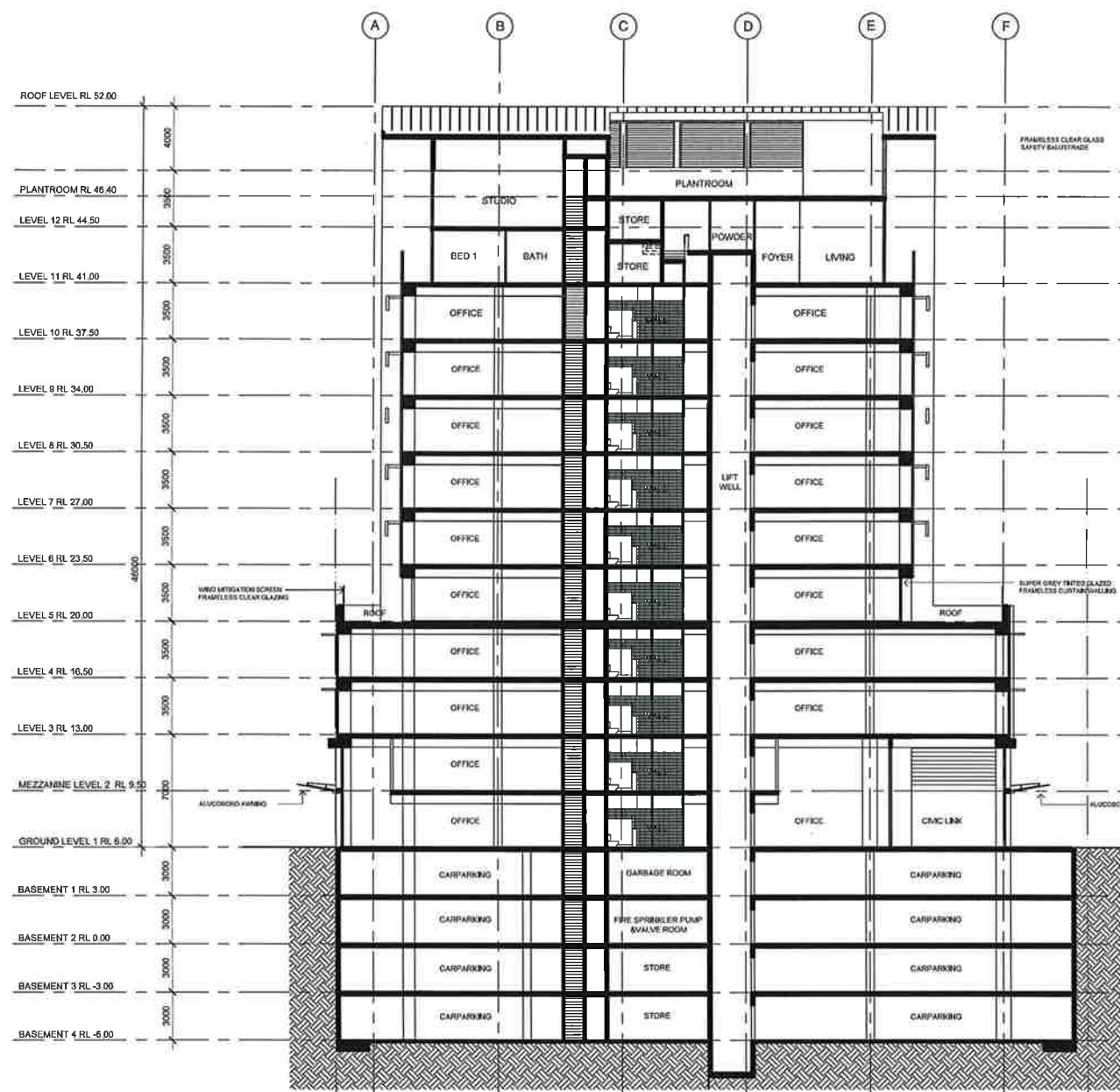
SECTION A - A Scale 1:200 @ A1
