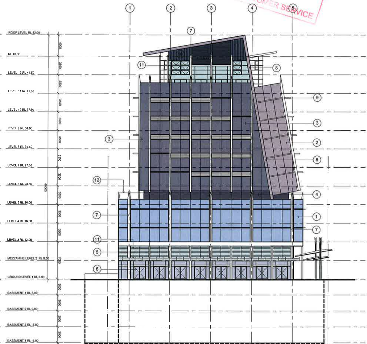
EASTERN ELEVATION Scale 1:200 @ A1
